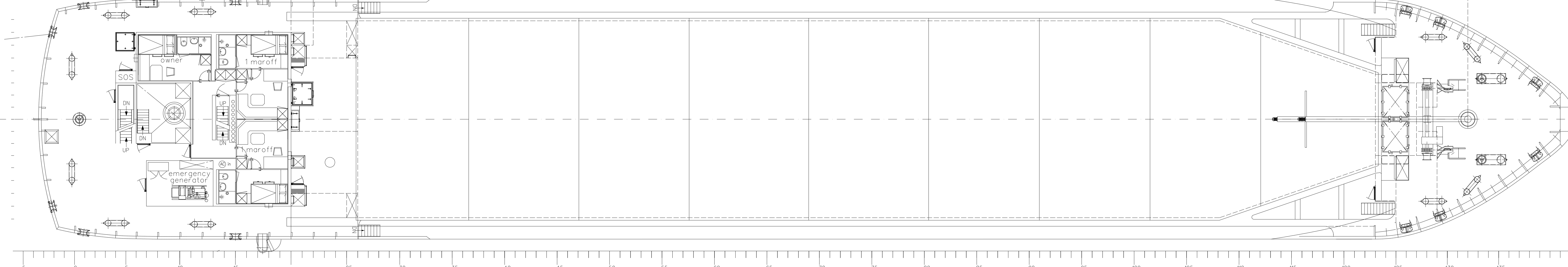
Main Deck
